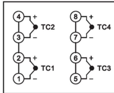
TC thermocouple input
