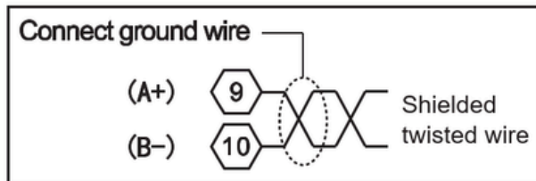
RS485 communication wiring diagram description
