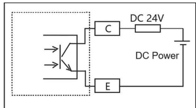
Transistor output wiring diagram description
